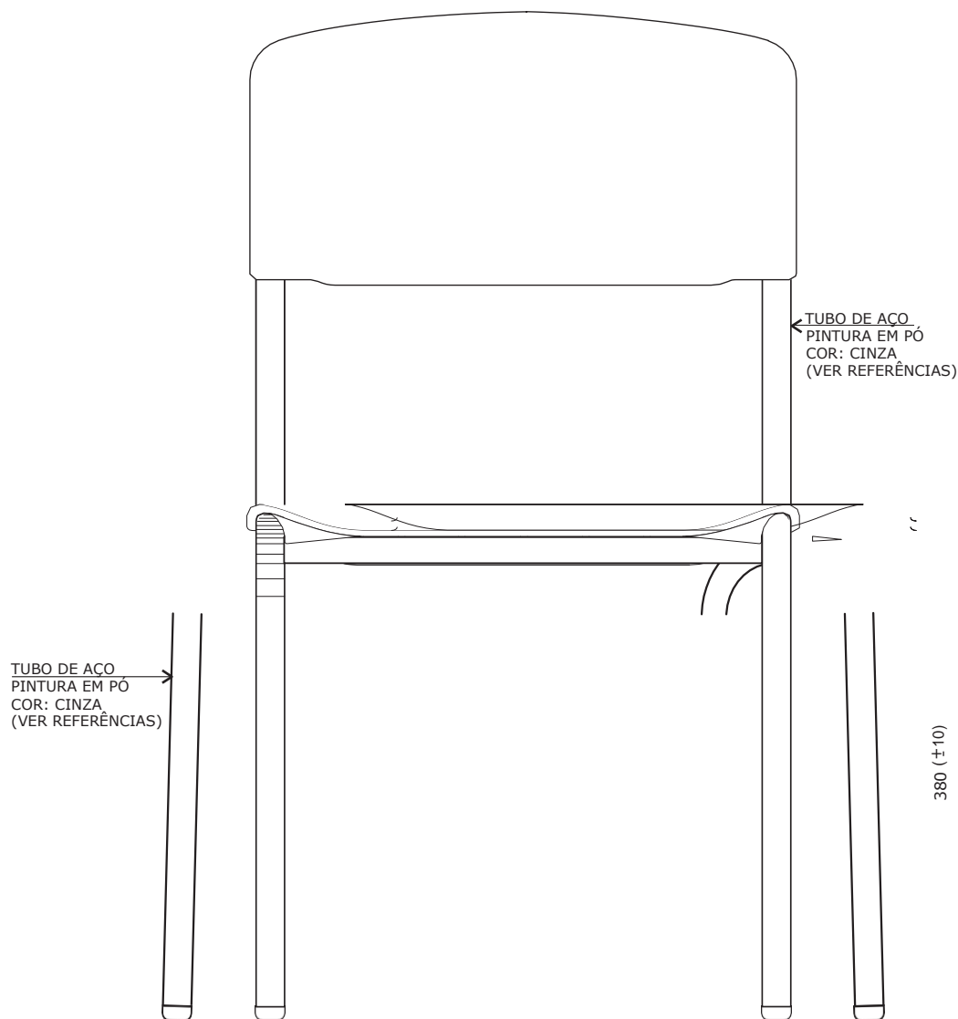
VISTA FRONTAL
